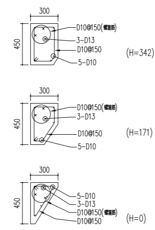
RC遮陽版配筋圖 Scale = 1/40
